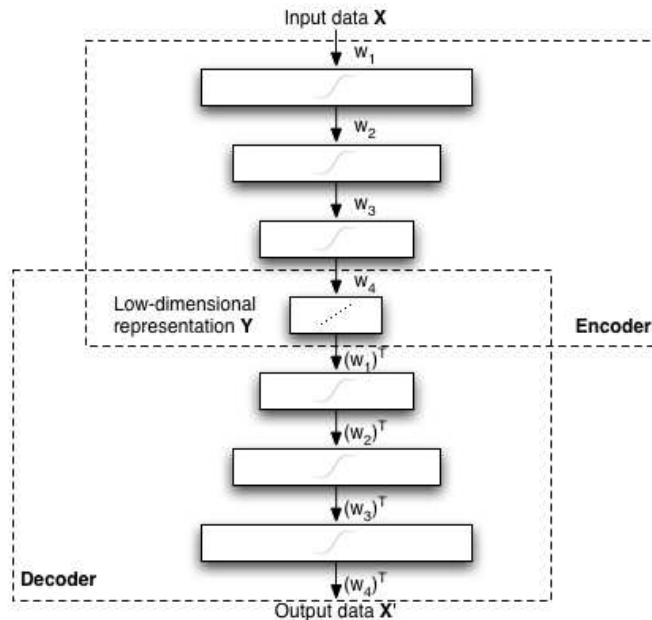
Figure 1: Schematic structure of an autoencoder.
